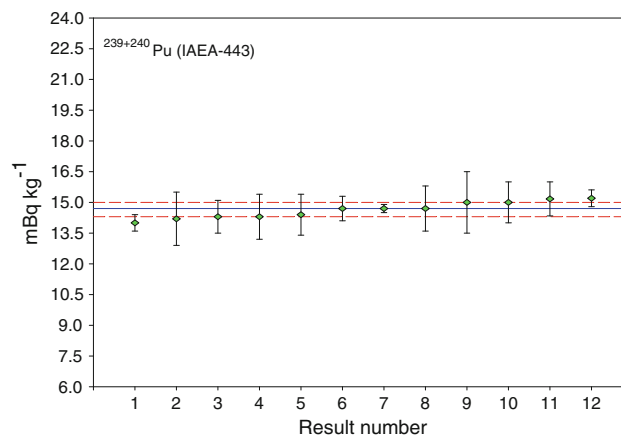
Fig. 5 Data evaluation for ^{239+240}\text{Pu} in IAEA-443. The median (solid line) and corresponding 95% confidence intervals (dashed lines) are shown. The error bars correspond to the combined uncertainty reported by laboratories
